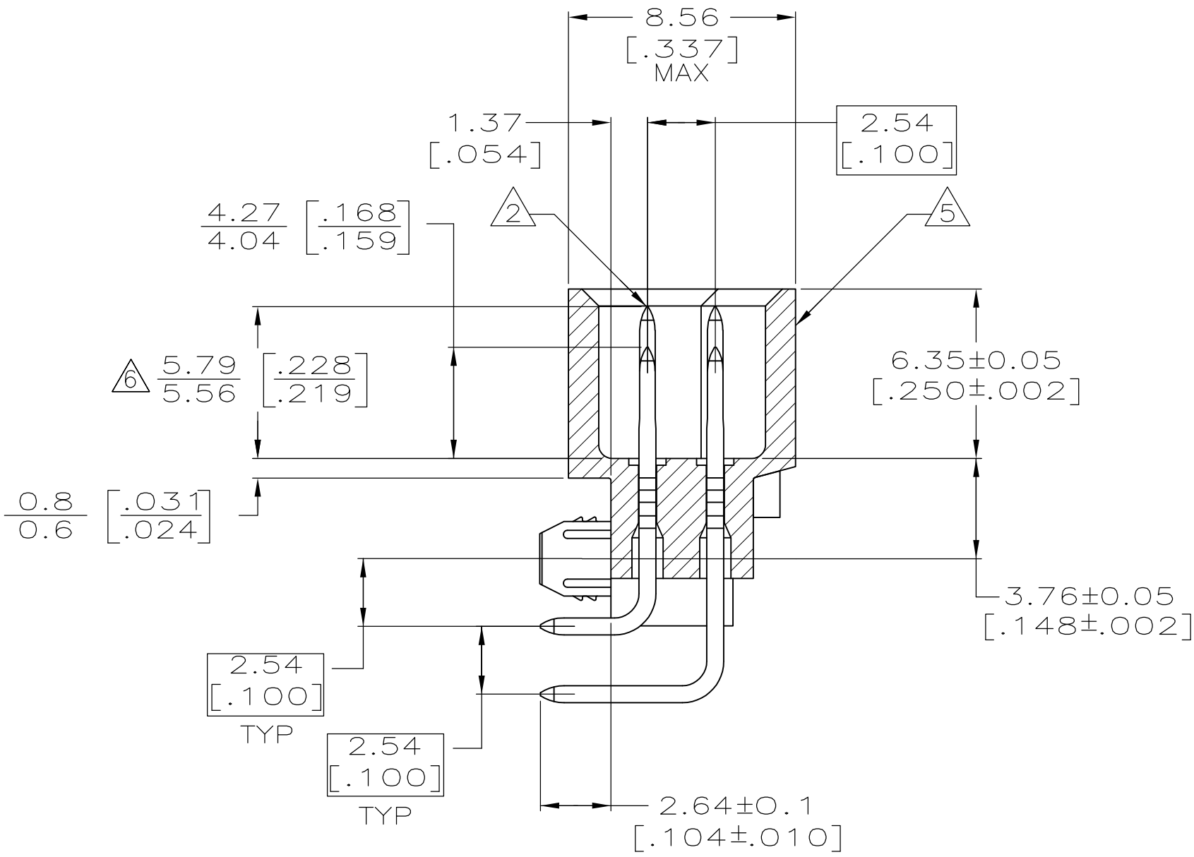
SECTION Z-Z
