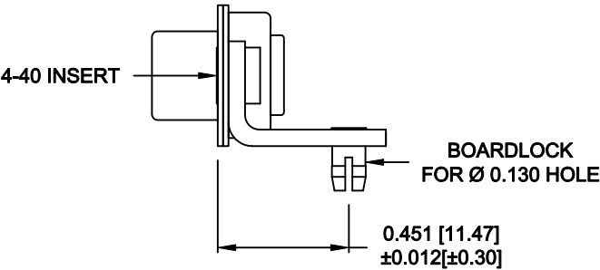
MOUNTING HARDWARE
