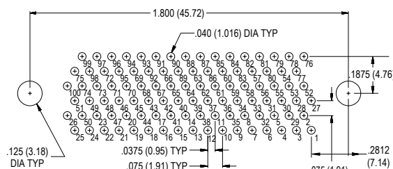
100 PIN MWDM-100PCBS
