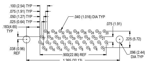
37 PIN MWDM-37PCBS
