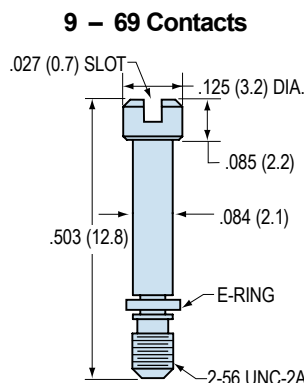
Kit Part Number 500-081-2 Kit Consists of 2 Jackscrews and 2 E-Rings
