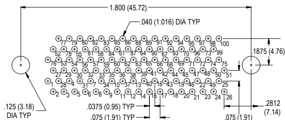
100 Socket MWDM-100SCBS
