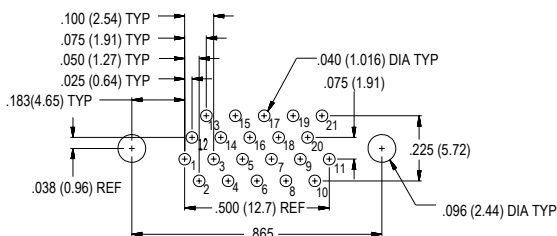
21 Socket MWDM-21SCBS
