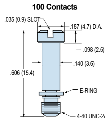
Kit Part Number 500-081-4 Kit Consists of 2 Jackscrews and 2 E-Rings
