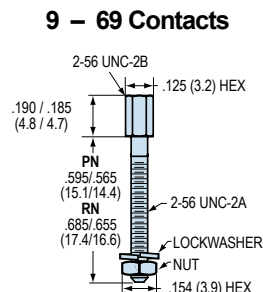
PN Kit Part Number 500-069-2-6 RN Kit Part Number 500-069-2-7 Kit Consists of 2 Jackposts, 2 Nuts, 2 Washers
