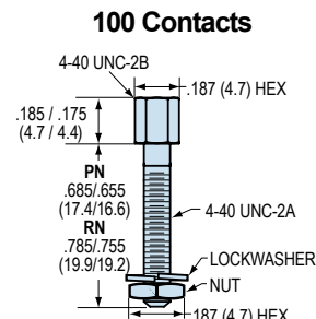
PN Kit Part Number 500-069-4-7 RN Kit Part Number 500-069-4-8 Kit Consists of 2 Jackposts, 2 Nuts, 2 Washers
