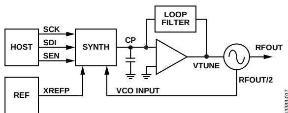
Figure 16. Typical Application Diagram
