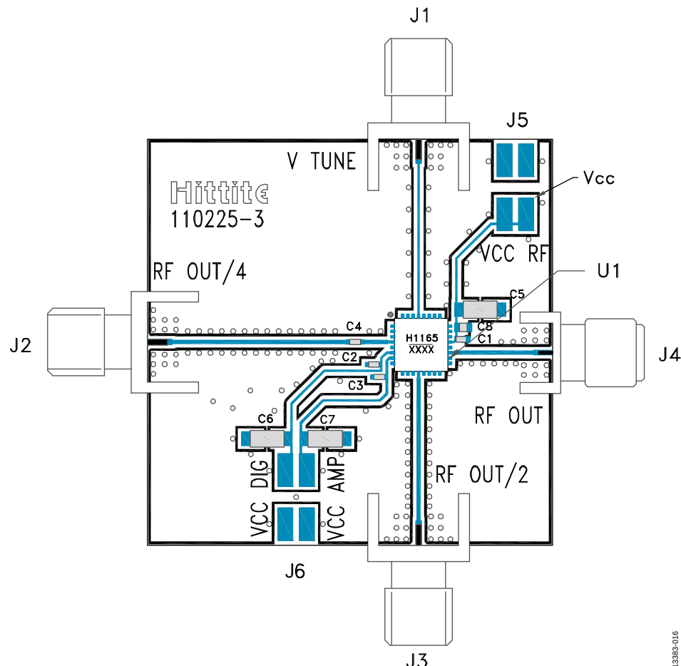
Figure 17. Evaluation Board
