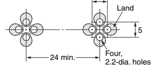
PCB-mounting Dimensions
