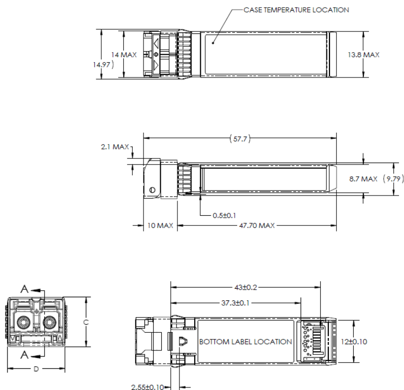
Figure 2. Mechanical Dimensions
