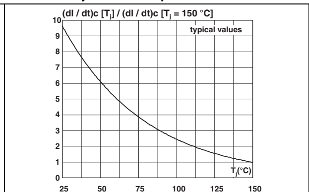
Figure 12. Relative variation of critical rate of decrease of current (di/dt) c versus junction temperature
