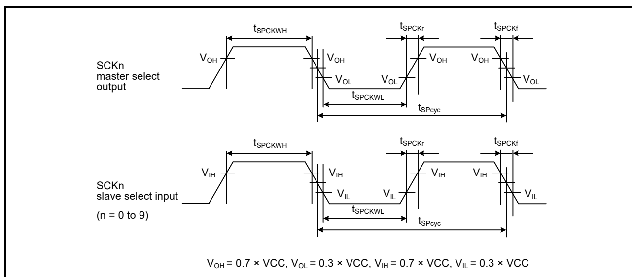
Figure 2.39 SCI simple SPI mode clock timing
