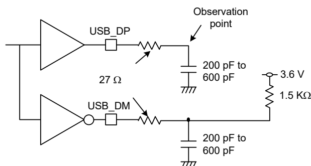
Figure 2.85 Test circuit in low-speed mode
