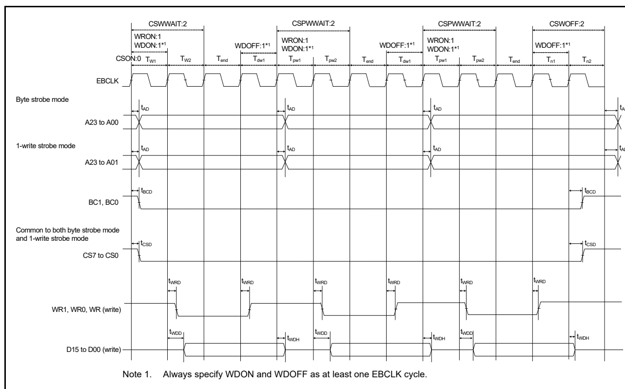
Figure 2.19 External bus timing for page write cycle with bus clock synchronized
