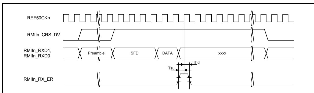
Figure 2.63 RMII reception timing when an error occurs
