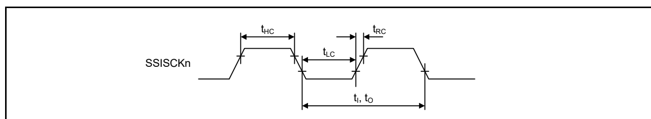
Figure 2.55 SSI clock input/output timing
