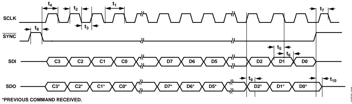
Figure 6. SPI Serial Interface Timing Diagram, CPOL = 0, CPHA = 1
