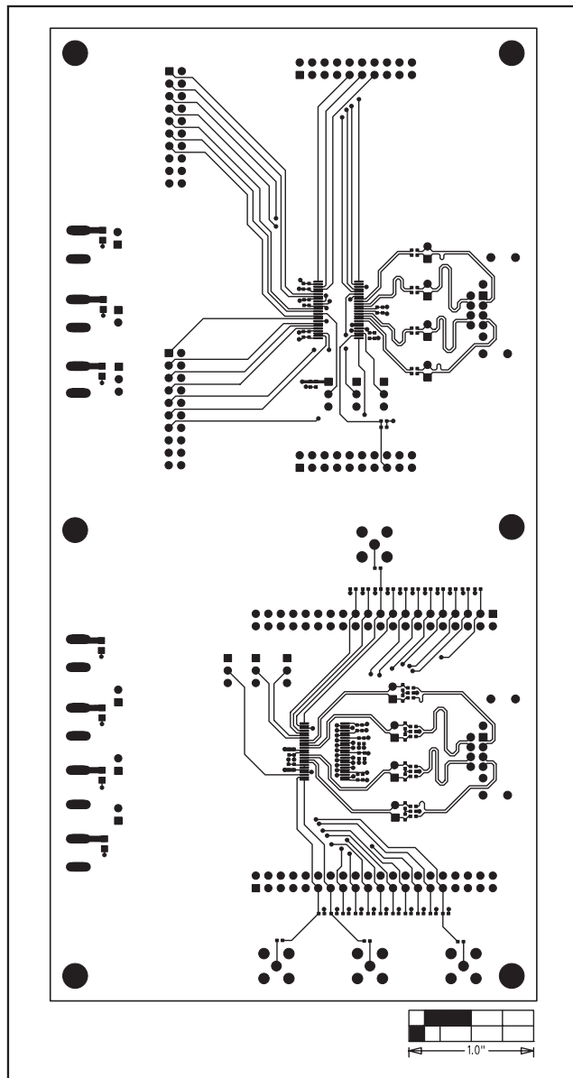
Figure 3. MAX9209/MAX9244 EV Kit PCB Layout—Component Side
