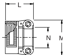
STYLE H Heavy Duty (Table IV)
