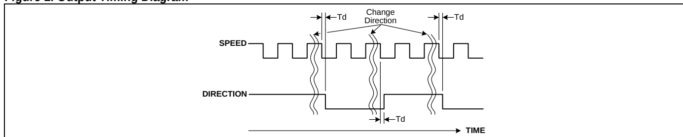
Figure 1. Output Timing Diagram
