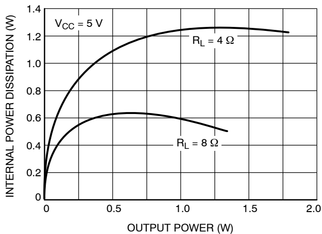
Figure 19. Power Dissipation vs. Output Power
