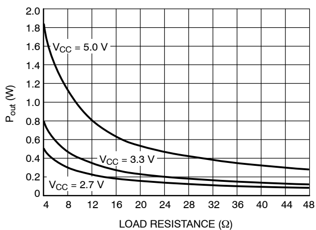
Figure 17. P_{OUT} vs. Load Resistance
