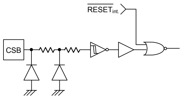
Figure 55. CSB input equivalent circuit
