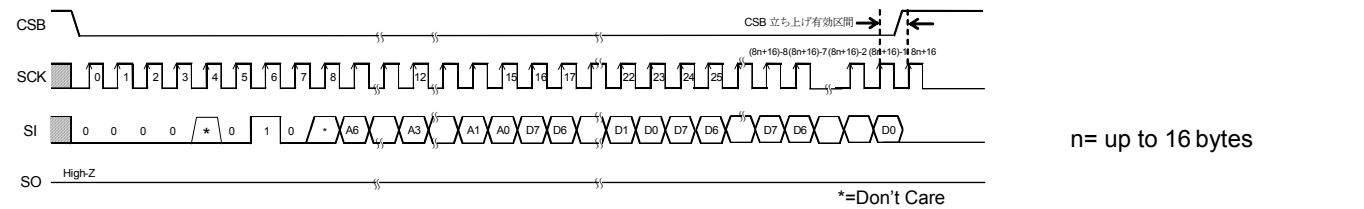
Figure 39. N Byte page write command
