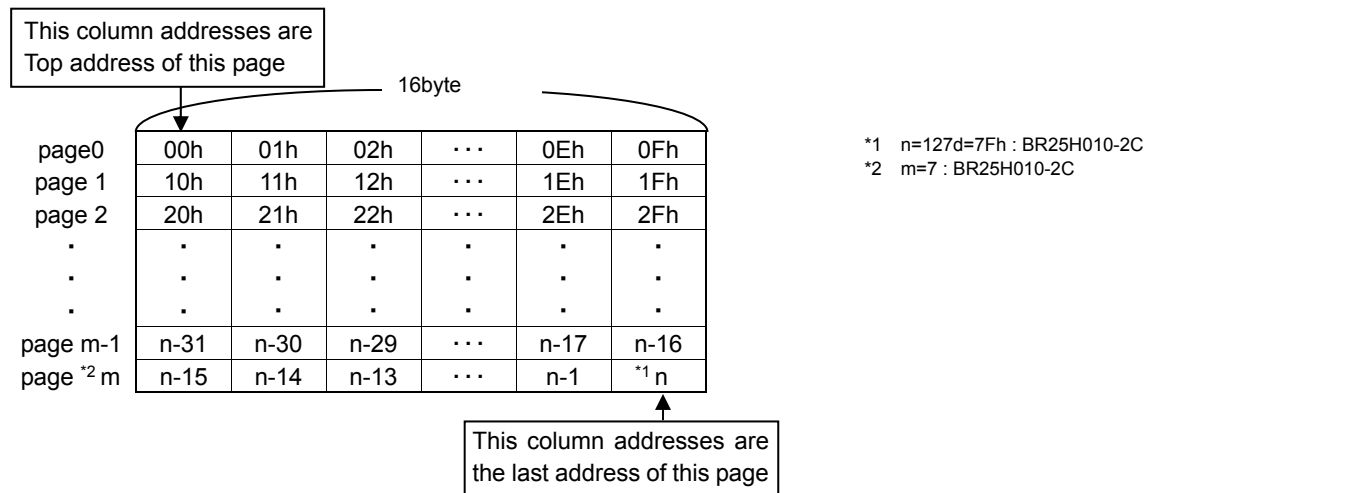
Figure 40. EEPROM physical address for Page write command (16Byte)
