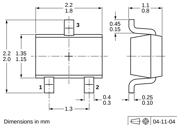
Fig 15. Package outline PDTC123JU (SOT323/SC-70)
