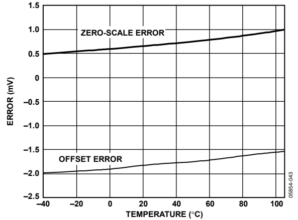
Figure 9. Zero-Scale Error and Offset Error vs. Temperature
