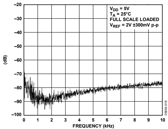
Figure 19. Total Harmonic Distortion
