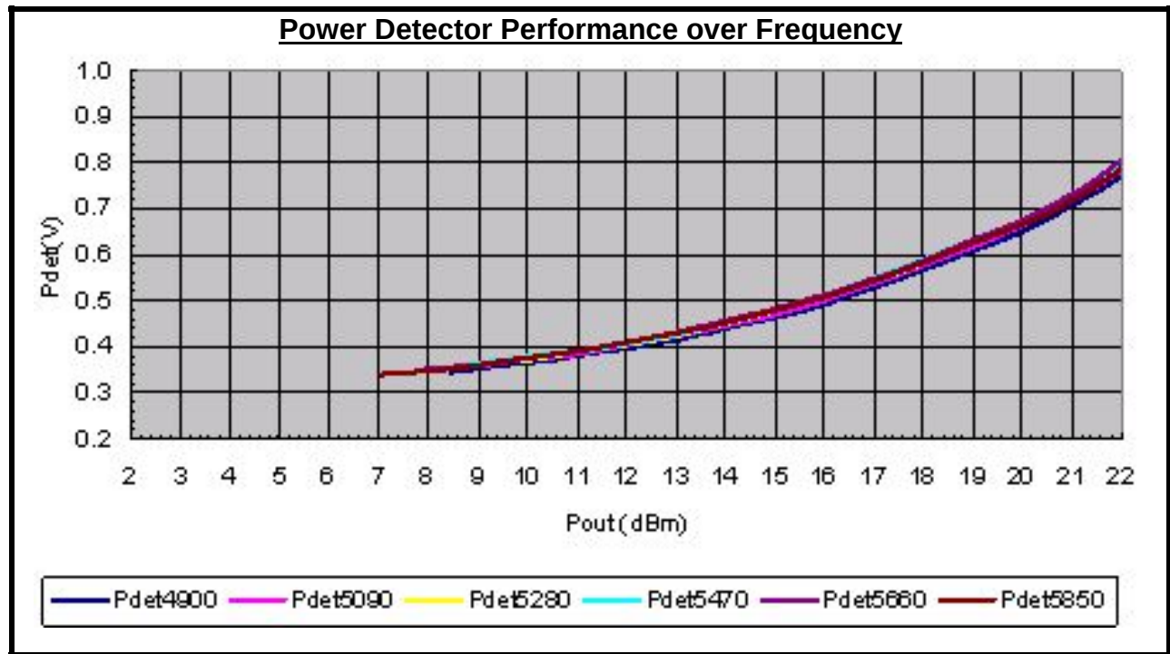
Figure 3: SE5007T Power Detector Characteristic
