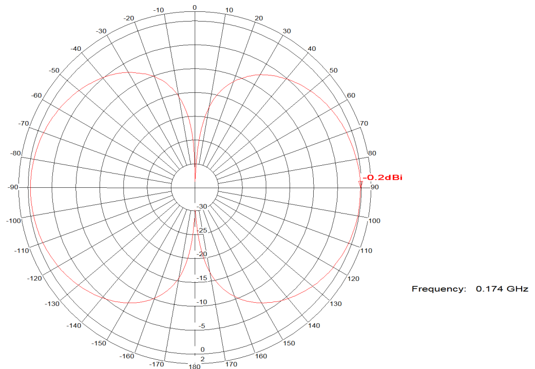
Figure 4: Azimuth & Elevation Gain Patterns @ 174 MHz
