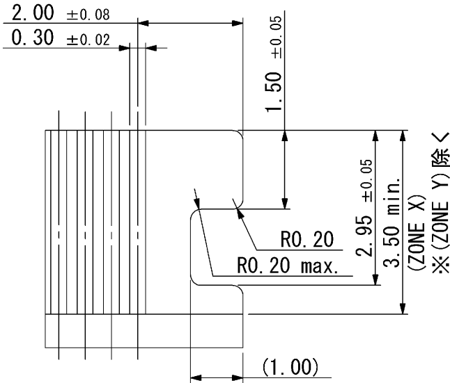
DETAIL D(S=10/1)
