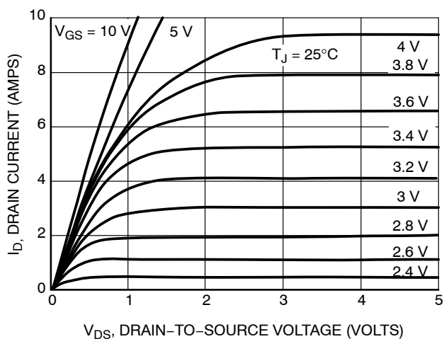
Figure 3. On-State Output Characteristics
