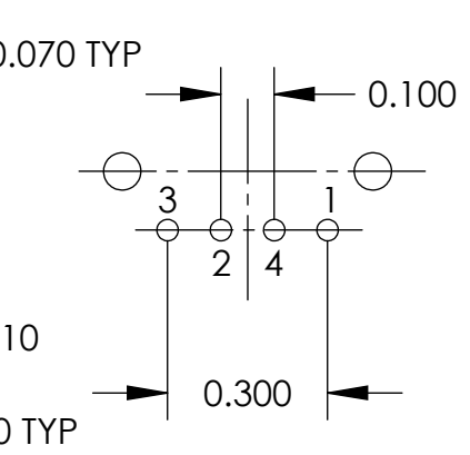
THRU HOLE TERMINATION (4 PIN) TRAPC4M1X TRAPC4MX
