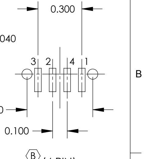
SMALL PROFILE SURFACE MOUNT (4 PIN) TRASM3MS1X TRASM3MSX
