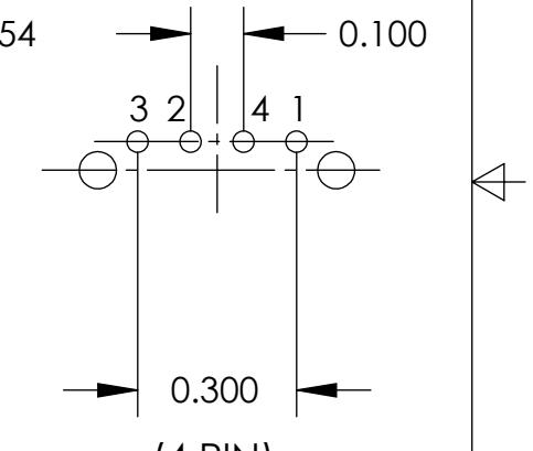
SMALL PROFILE THRU HOLE TERMINATION (4 PIN) TRAPC4MS1X TRAPC4MSX
