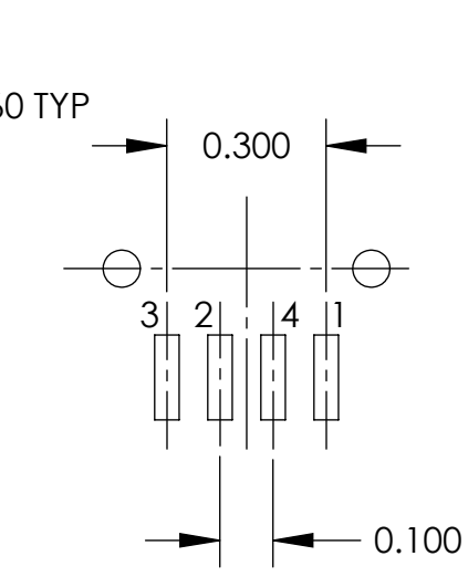
SURFACE MOUNT (4 PIN) TRASM4M1X TRASM4MX
