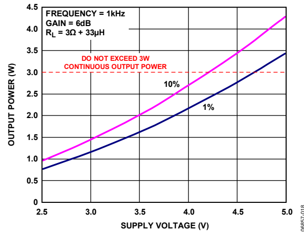
Figure 18. Maximum Output Power vs. Supply Voltage, R_L = 3\Omega + 33\mu H , Gain = 6 dB
