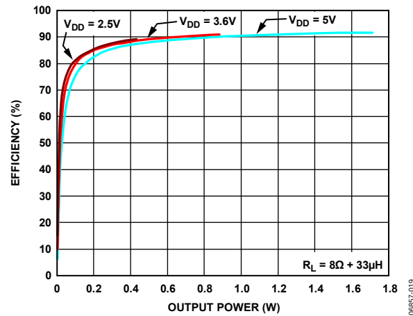
Figure 19. Efficiency vs. Output Power, R_L = 8\Omega + 33\mu H
