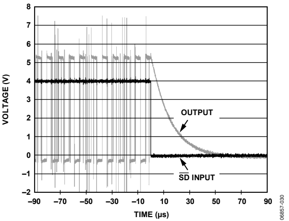
Figure 30. Turn-Off Response
