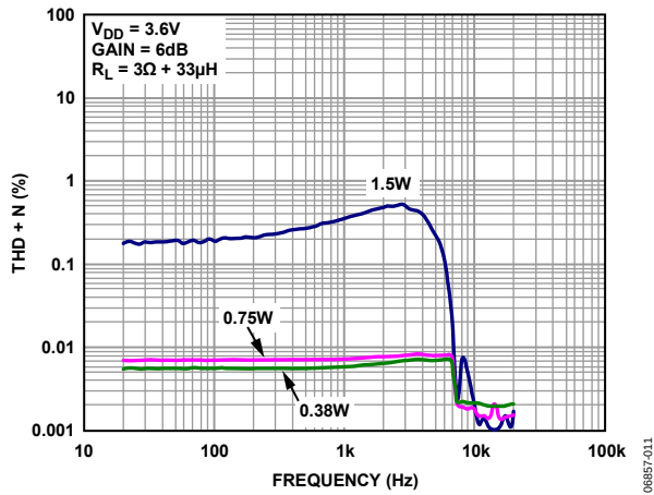
Figure 11. THD + N vs. Frequency, V_{DD} = 3.6V , R_L = 3\Omega + 33\mu H , Gain = 6 dB
