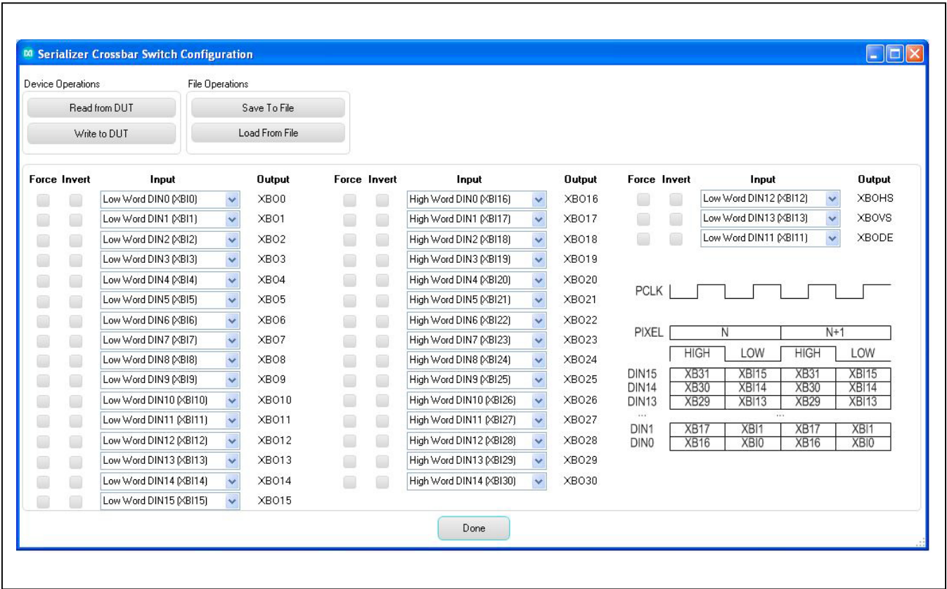
Figure 8. MAXSerDesEV-N EV Kit Software: Evaluation Kit Window (Serializer Crossbar Switch Configuration Window)
