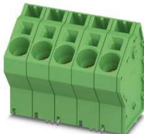
30° angled connection direction, zigzag pinning, 600 V UL approval
