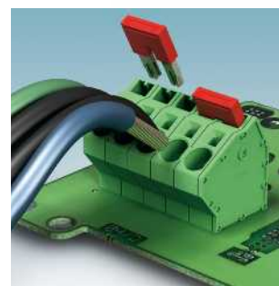
Angled PCB terminal blocks with push-in spring connection up to 6 mm 2 , 10 mm pitch SPTA 16/ ...-10,0-ZB Page 27
