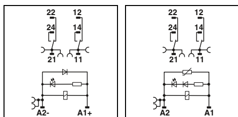
DC coils
