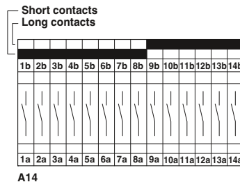
6 (10) mm², 30 A, test terminal strip, for wall mounting, VDE coded type A14
