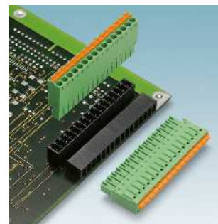
Single-level headers, 13 to 20-pos., for reflow processes, 3.81 mm pitch MC 1,5/ ...-G-3,81 P20 THR Page 18 MCV 1,5/ ...-G-3,81 P20 THR Page 19
