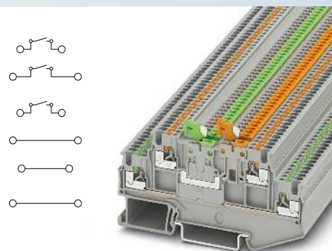
1.5 (1.5) mm², 8 A, double-level knife disconnect terminal block, four connections, not bridgeable
