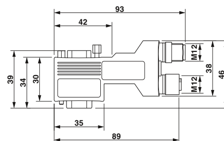
SUBCON-PLUS...90X...M12 dimensional drawing, long 90° version
