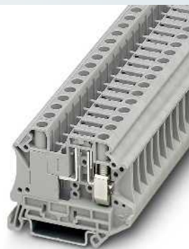
6 (10) mm 2 , 20 A, disconnect terminal block, with test socket screws
