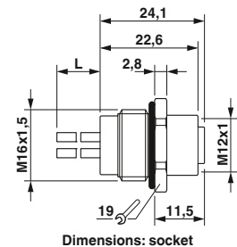
Dimensions: socket
