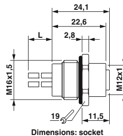
Dimensions: socket
