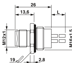
Dimensions: plug
