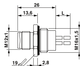
Dimensions: plug
