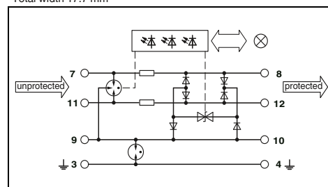
3-wire with common reference potential, 9/10 connection grounded via gas-filled surge
