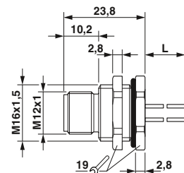
Dimensions: plug
