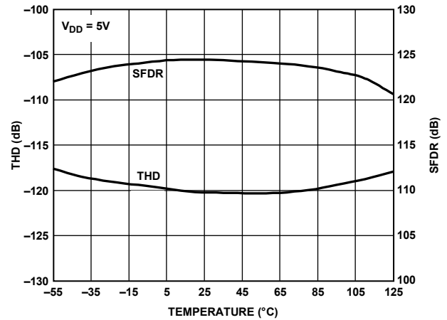
Figure 17. THD, SFDR vs. Temperature
