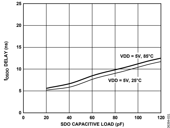
Figure 24. t_{\text{DSO}} Delay vs. Capacitance Load and Supply
