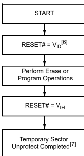
Figure 3. Temporary Sector Unprotect Operation
