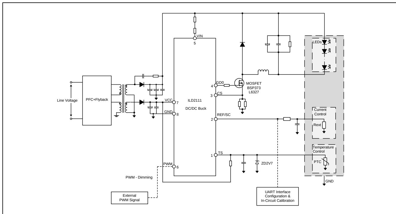
Figure 1. Typical Application
