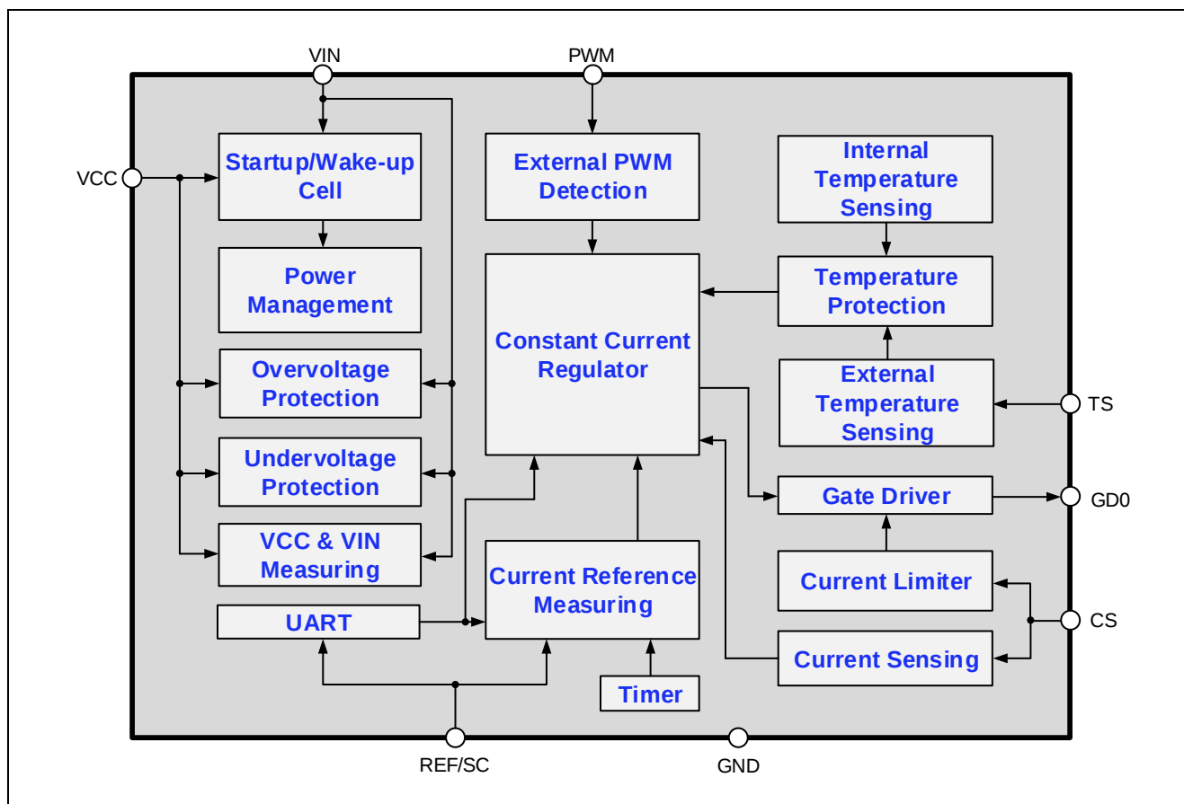
Figure 3. Block Diagram
