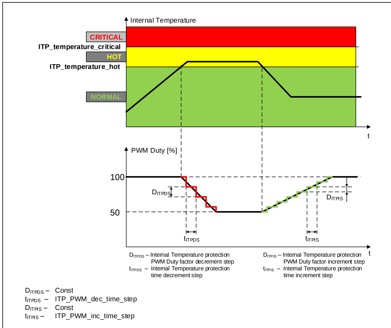
Figure 24. Internal Temperature Protection
