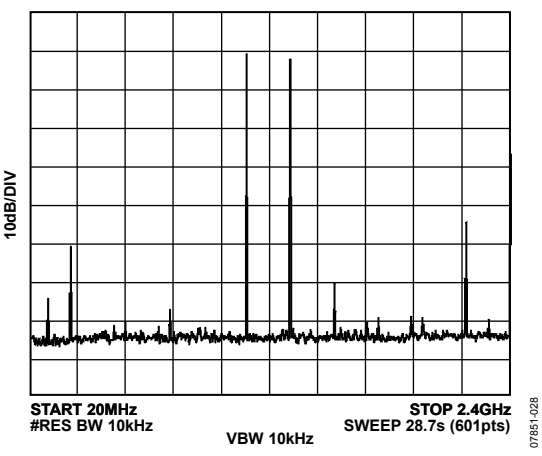
Figure 28. Single-Tone Spectrum in Mix Mode at f_{OUT} = 1.31 GHz, f_{DAC} = 2.4 GSPS
