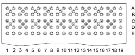
Recommended PCB hole mounting pattern for row differential applications
