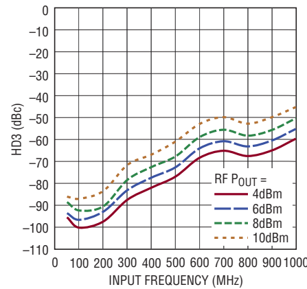
HD3 vs Input Frequency Over P_{OUT}
