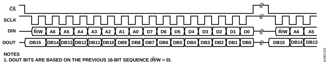
Figure 16. Example SPI Read Sequence
