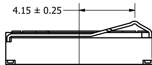
Side View (2)
