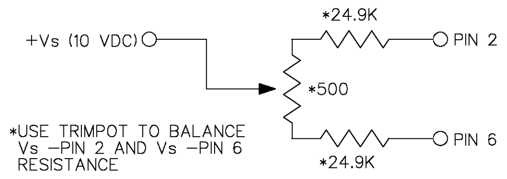
SENSING BRIDGE SUPPLY CIRCUIT
