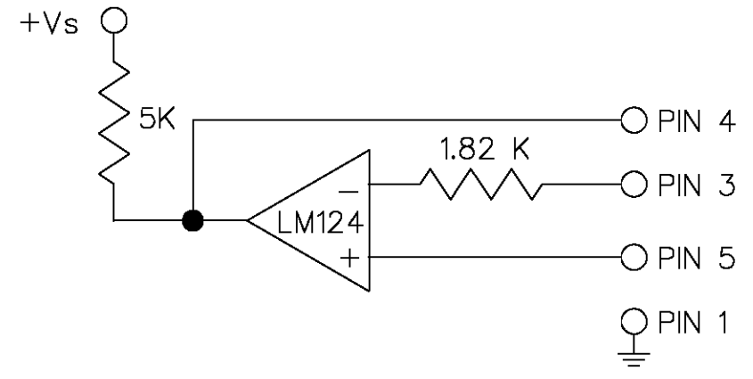
HEATER CONTROL CIRCUIT
