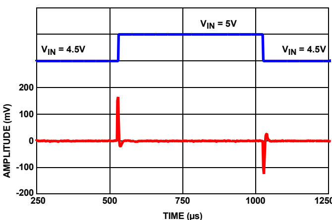
FIGURE 92. LINE TRANSIENT WITH 0.1\mu F LOAD
