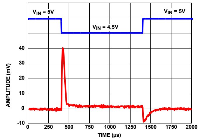
FIGURE 127. LINE TRANSIENT RESPONSE WITH 10μF LOAD
