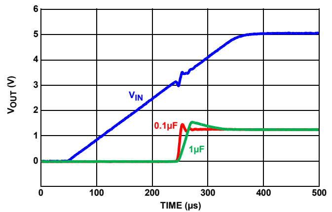
FIGURE 29. TURN-ON TIME
