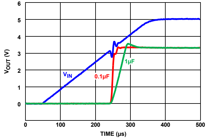
FIGURE 114. TURN-ON TIME
