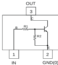
Device Schematic
