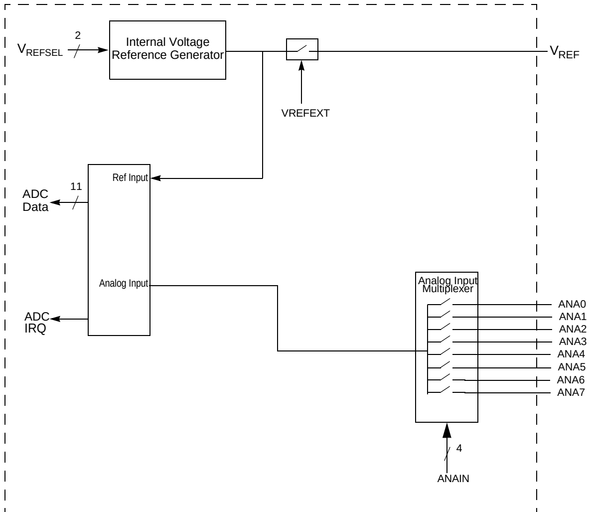
Figure 19. Analog-to-Digital Converter Block Diagram
