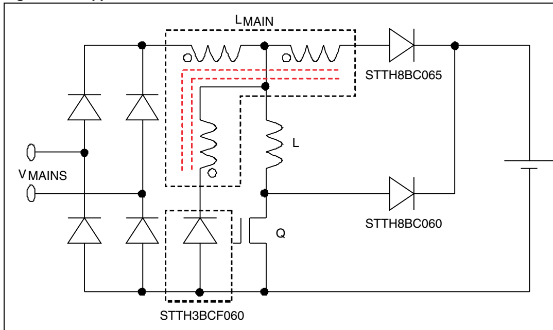
Figure 13. Application schematic
