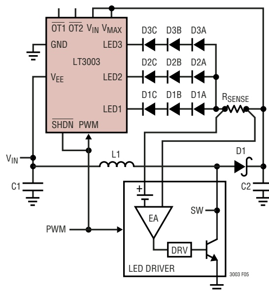
Figure 5. Buck-Boost Mode
