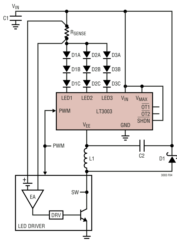
Figure 4. Buck Mode
